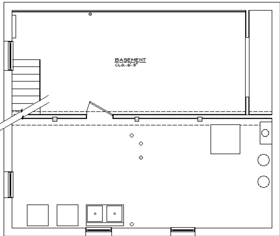
BASEMENT PLAN
